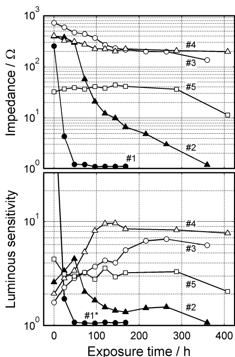
Time courses of the measured dark impedances (top panel) and luminous sensitivities (bottom). Each line corresponds to the coating and test condition indicated and numbered in Table 1. *: The luminous sensitivity value of the electrode #1 at 0 h was about 200 and out of the range shown.
